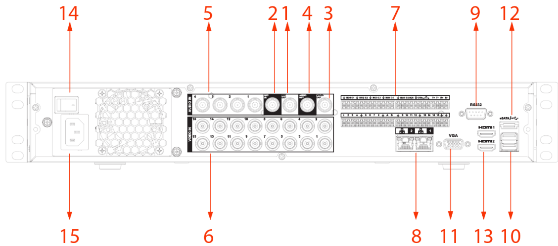
Figure 3-20 Rear panel (3)
