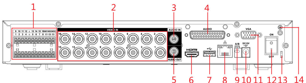
Figure 3-12 Rear panel
