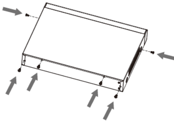
Figure 2-29 Fasten screws
