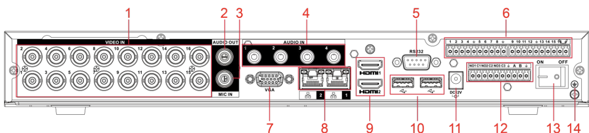
Figure 3-15 Rear panel
